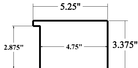
Large Termination Trim
