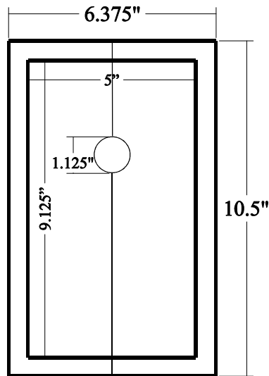
Low Profile Faucet Mounting Block
