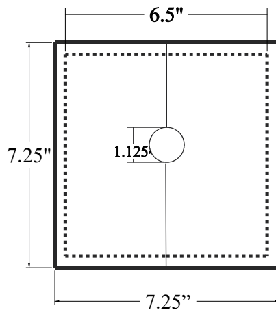
Faucet Mounting Block
