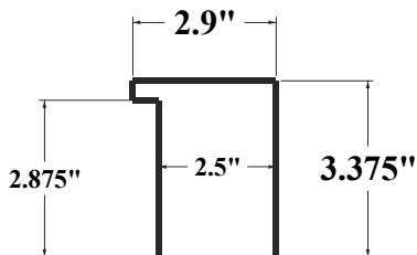
Standard Termination Trim
