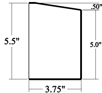
Large Window Sill/Head Trim
