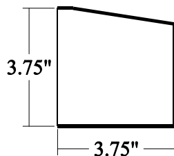
Small Window Sill/Head Trim
