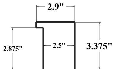
Standard Casing Trim With Flange
