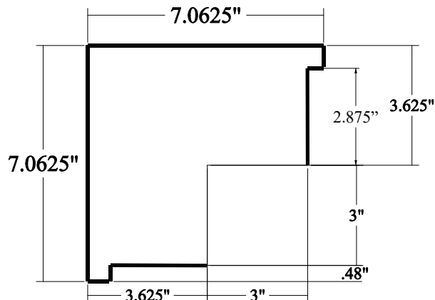
Square Outside Corner
