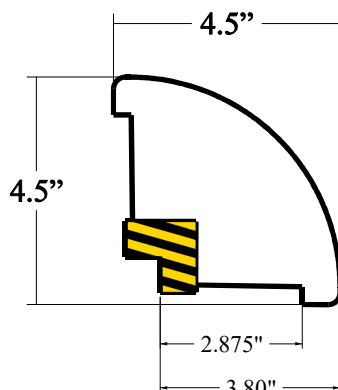
Round Outside Corner
