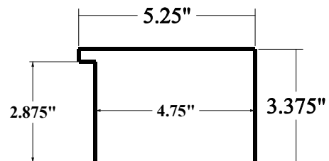
Large Casing Trim With Flange
